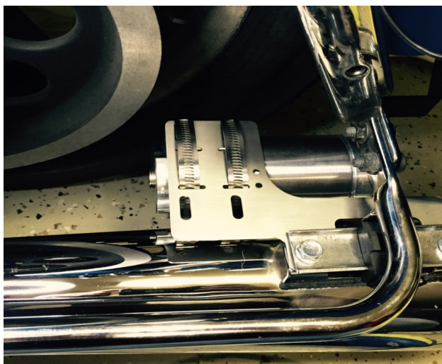
Air Tank and Compressor Mounted
