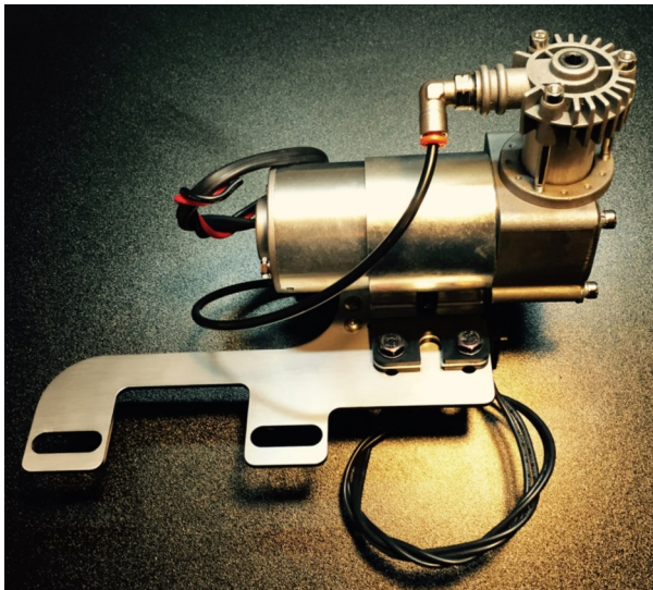
Compressor and air valve mounted on the bracket
