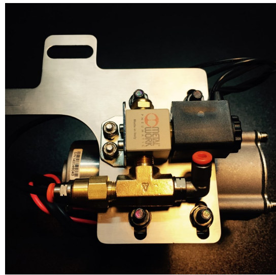
Compressor and air valve mounted on the bracket
