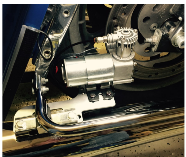
Air Tank and Compressor Mounted
